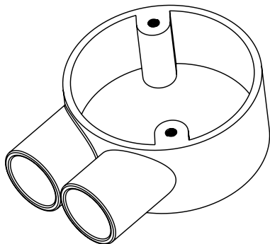
M4 Brass thread Isometric view
